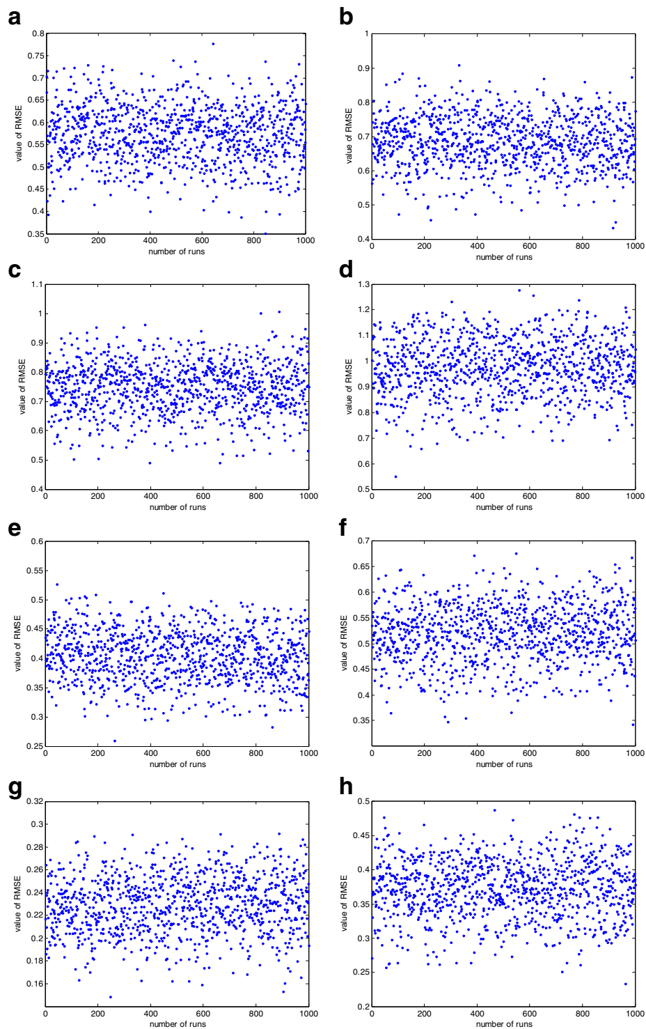
Fig. 2 the RMSEs of 1000 simulation runs for noise free and noisy scenarios. The figures in left column represent the noise free scenario in a IUKF, c SA, e PSO, g DPSO. The figures in the right column correspond to noisy scenario in b IUKF, d SA, f PSO and h DPSO
